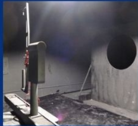
DISTRIBUTION PHOTOMETER
